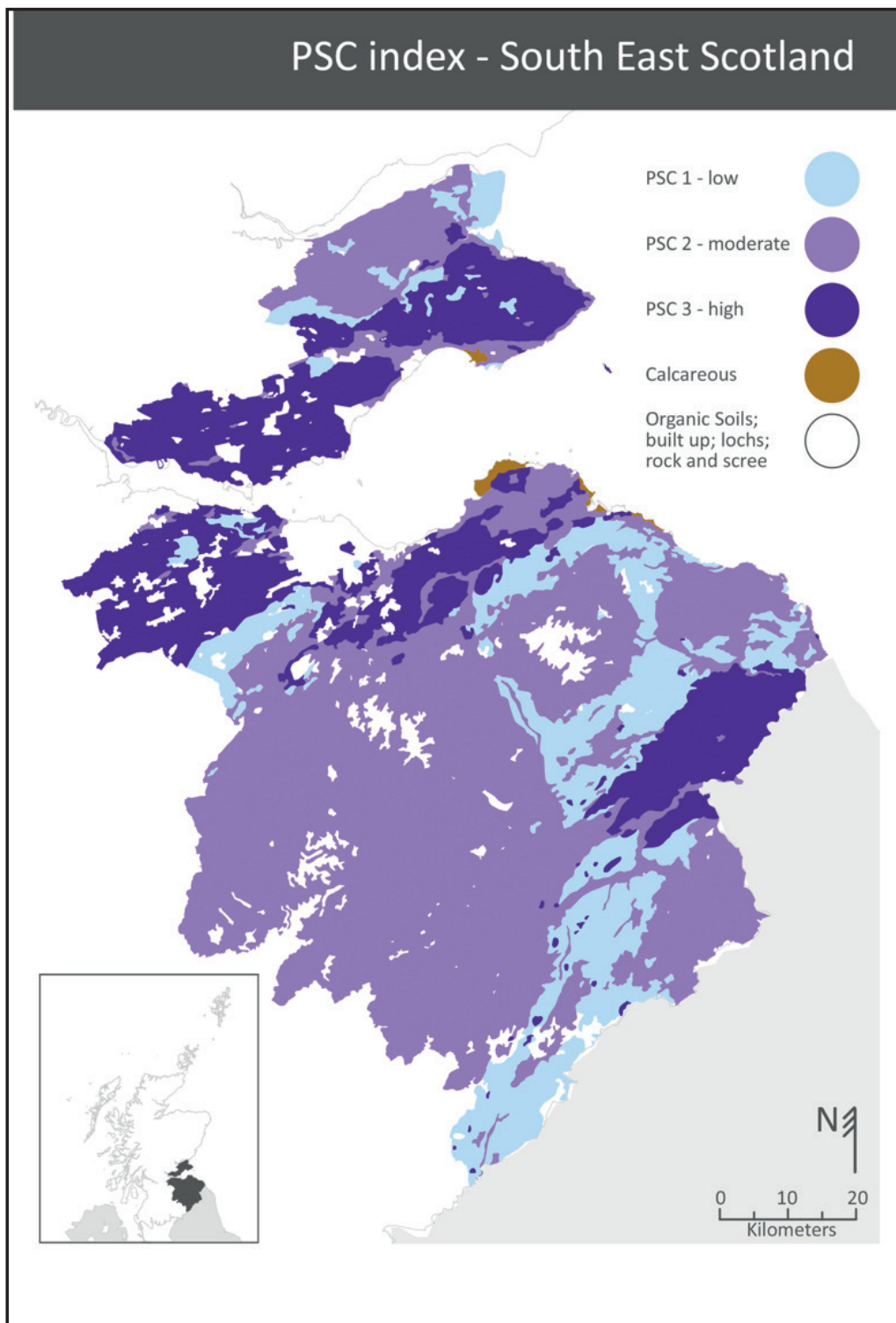
Figure 1. Map of P sorption capacity (PSC) from index 1 to 3 by soil association for non-calcareous mineral soils in SE Scotland.
